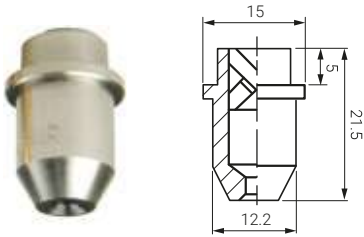
Outer shape of BX 1508 - BX 1743
