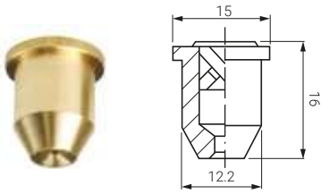
Outer shape of BX 1149 - BX 1372
