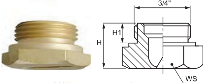
3/4" Large capacity
