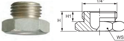
1/4" Standard capacity
